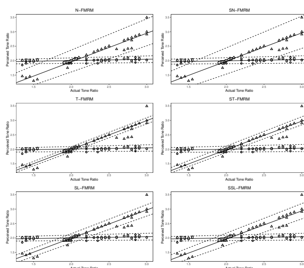
Figure 2: Tone perception data scatterplot and the fitted SMSN-FMRM models.
