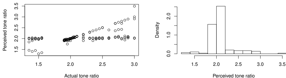
Figure 1: Tone perception data scatterplot and histogram.
