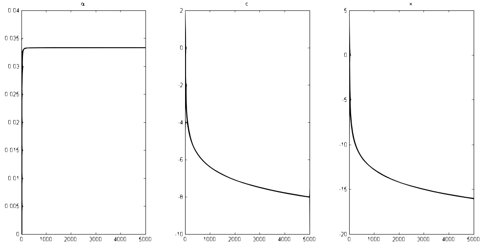
Figure 1: Plots of the score functions with (\alpha, c, k) = (30, 2, 1)
