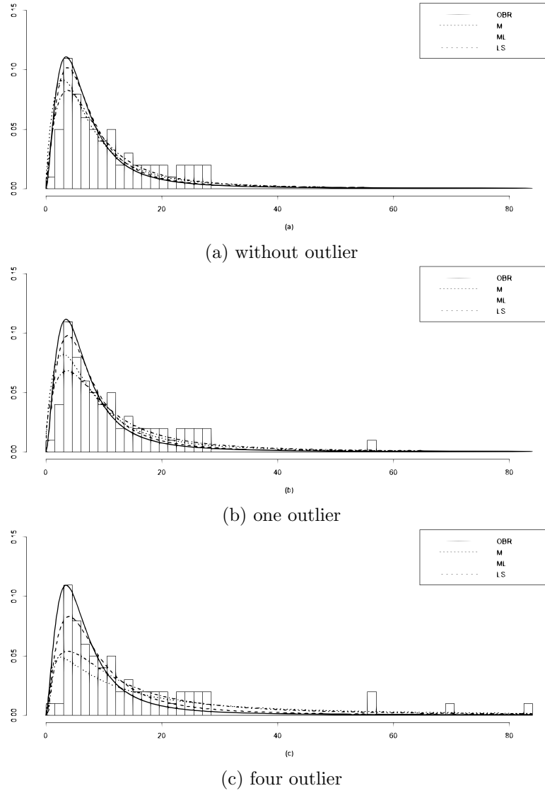
Figure 2: Histogram of Ibuprofen data and the fitted densities with the ML, LS, robust M and OBR estimates
